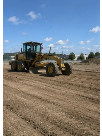
Photo #3. Ground clearing and leveling completed
