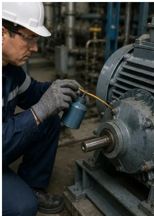
Photo #11. Lubrication work performed on equipment components
