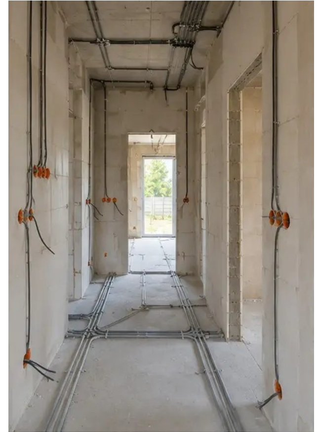
Photo #9 Electrical systems installation in progress
